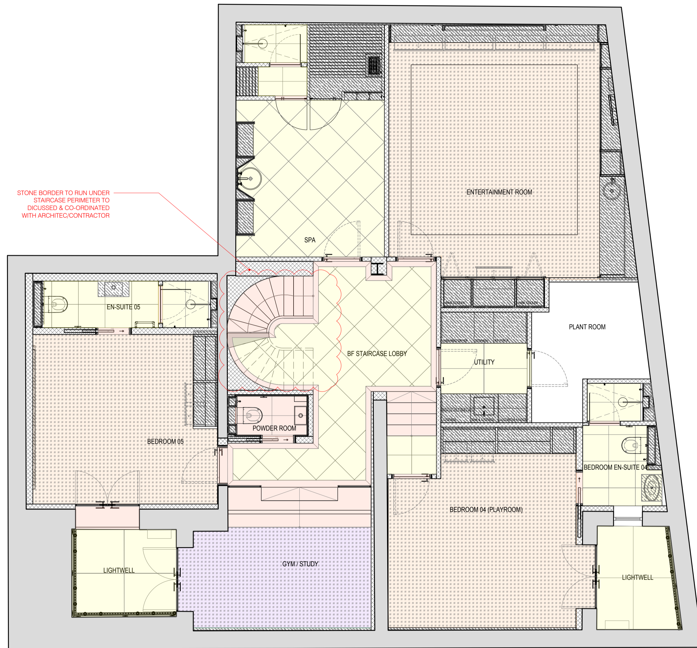
00 BF FLOOR FINISHES PLAN Scale 1:50
