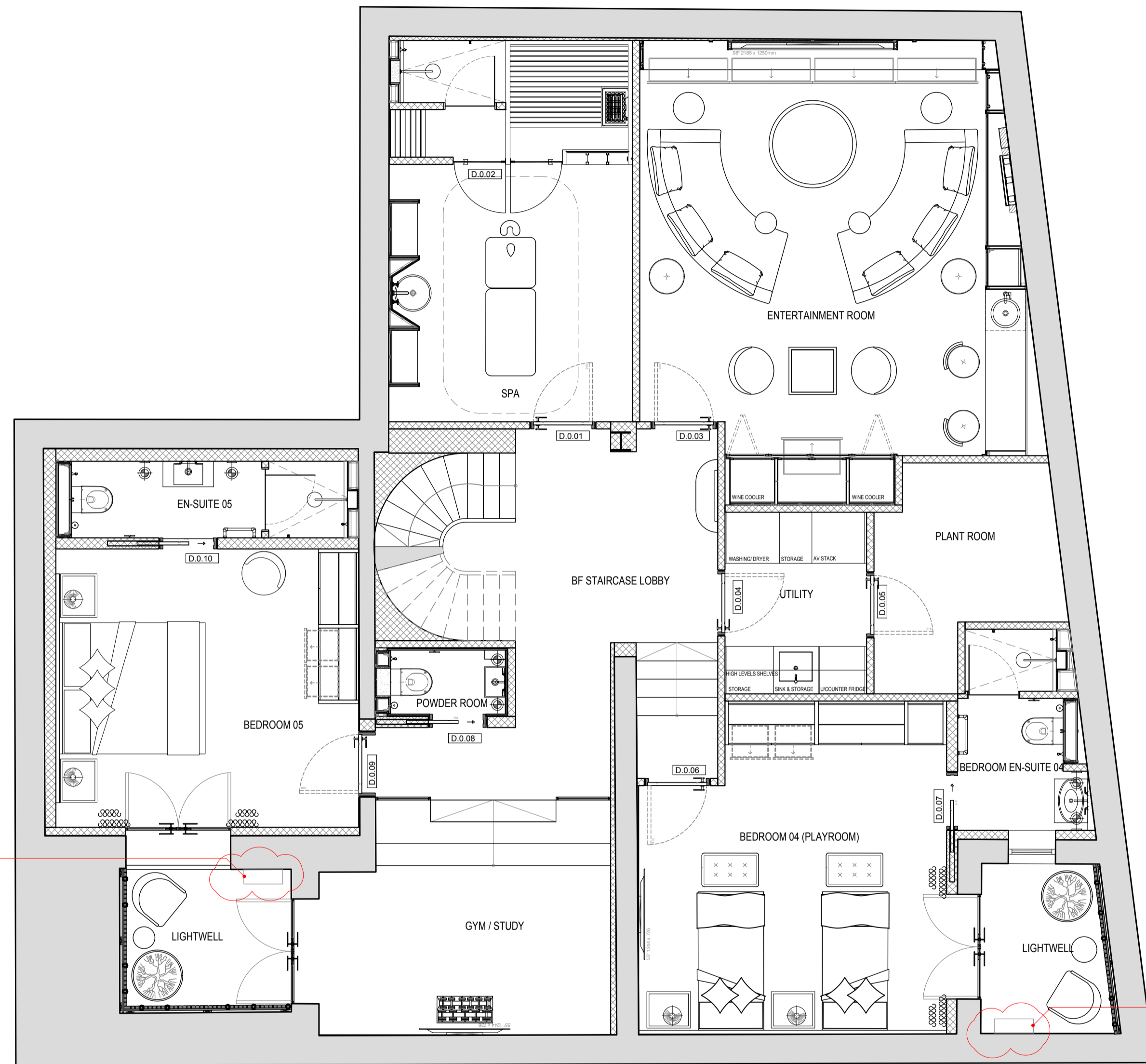
00 BF GA PLAN Scale 1:50
