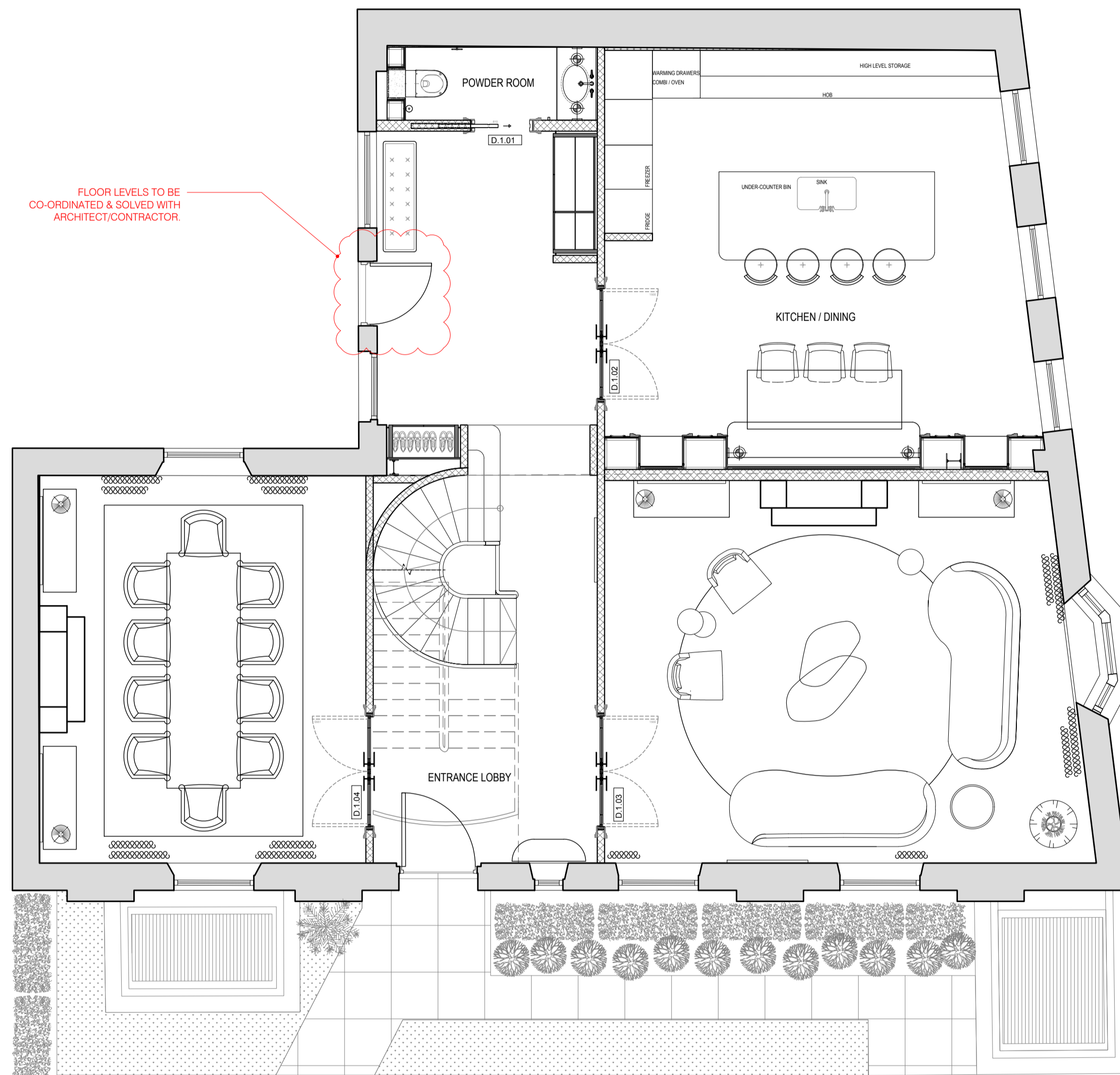
00 GF GA PLAN Scale 1:50
