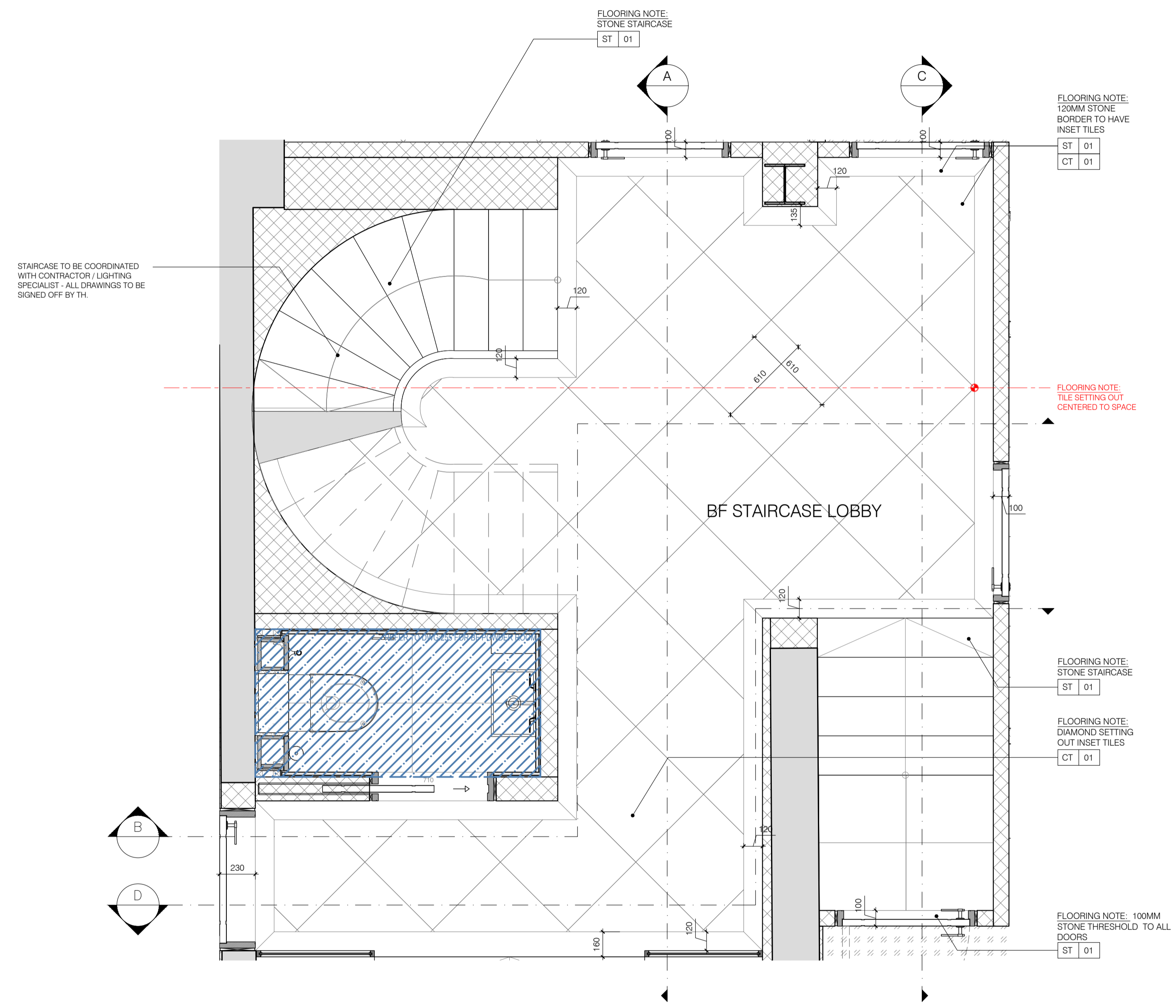
00 BF STAIRCASE LOBBY PLAN Scale 1:20
