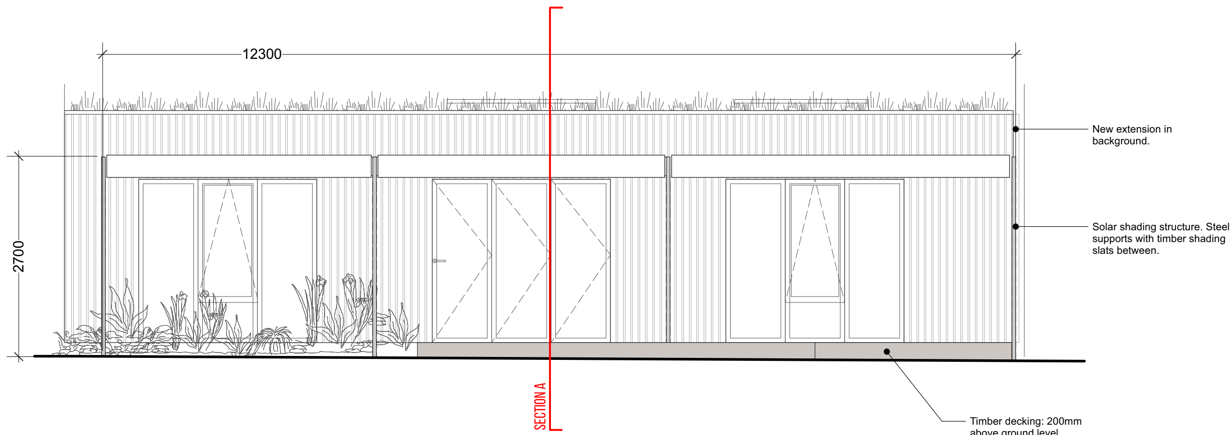
PROPOSED FRONT (SOUTH) ELEVATION B SCALE 1:50 @ A3
