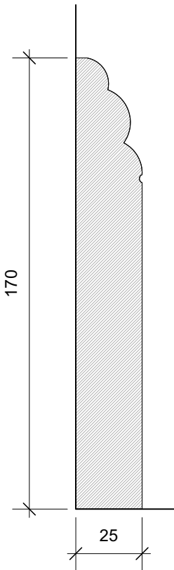
SK01 SKIRTING PROFILE Scale: 1:2
