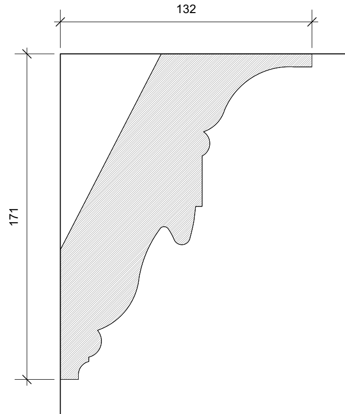
CN01 CORNICE PROFILE Scale: 1:2
