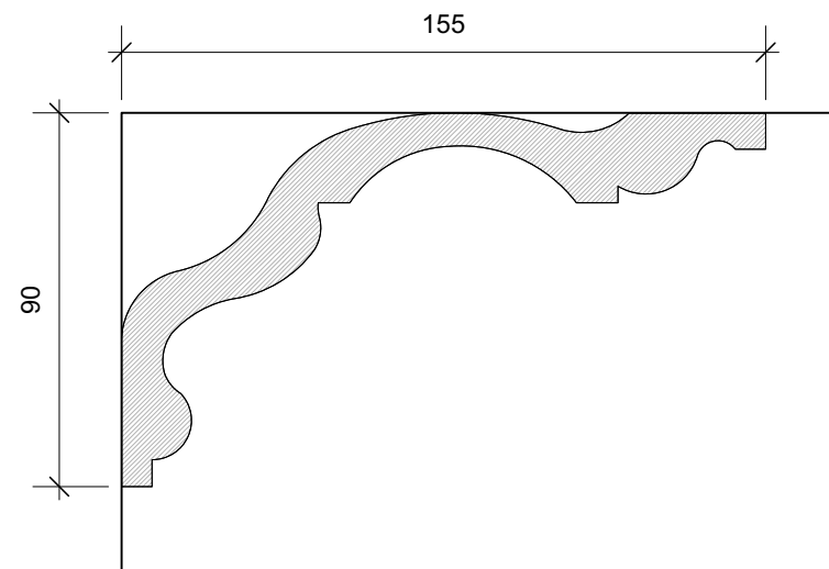
CN01 CORNICE PROFILE Scale: 1:2
