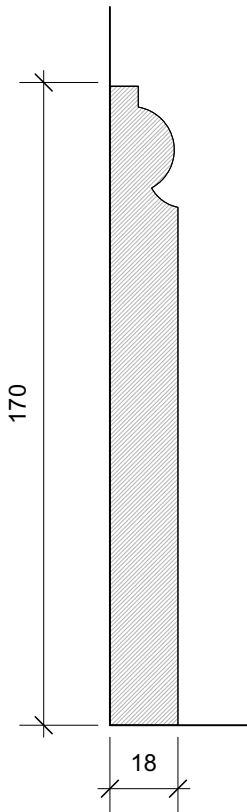
SK02 SKIRTING PROFILE Scale: 1:2
