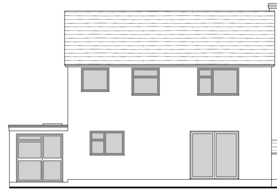
SOUTH / REAR ELEVATION
