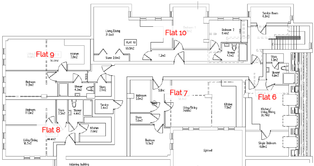
Second Floor as Proposed
