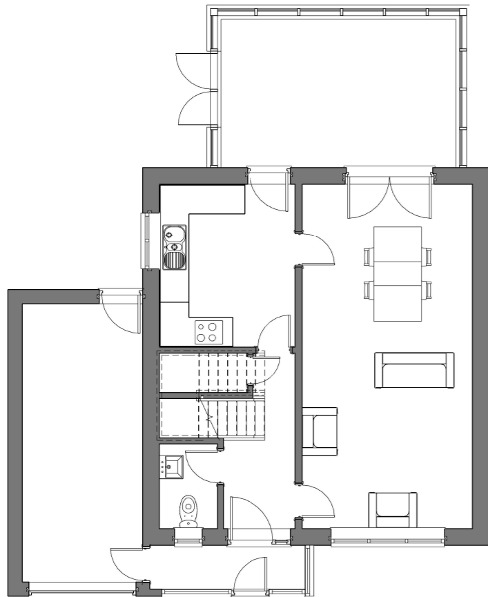
1 Existing Ground Floor Plan 1 : 50
