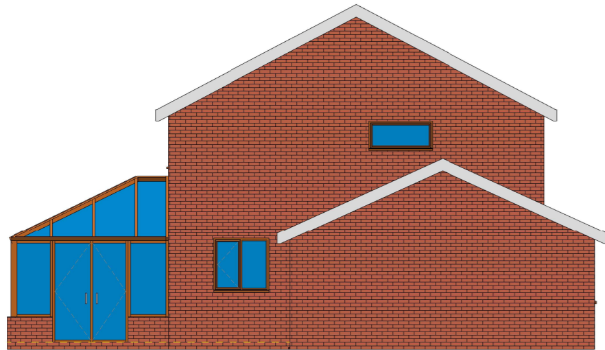
3 Existing LHS Gable Elevation 1 : 50
