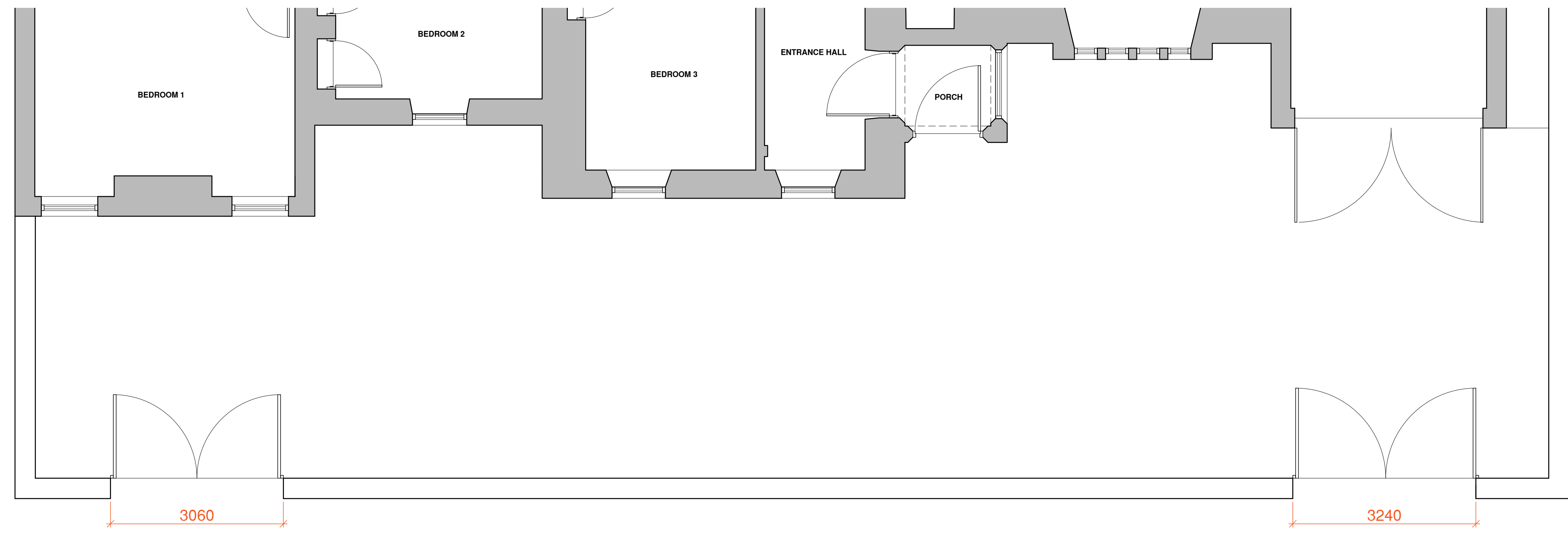
ENTRANCE PLAN AS EXISTING SCALE 1:50
