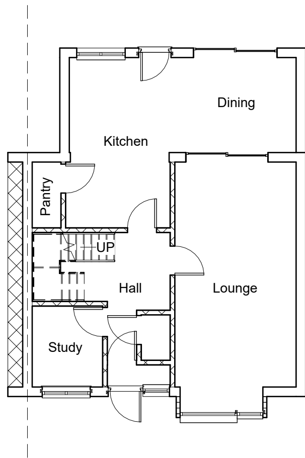
1 Existing Ground Floor 1 : 100
