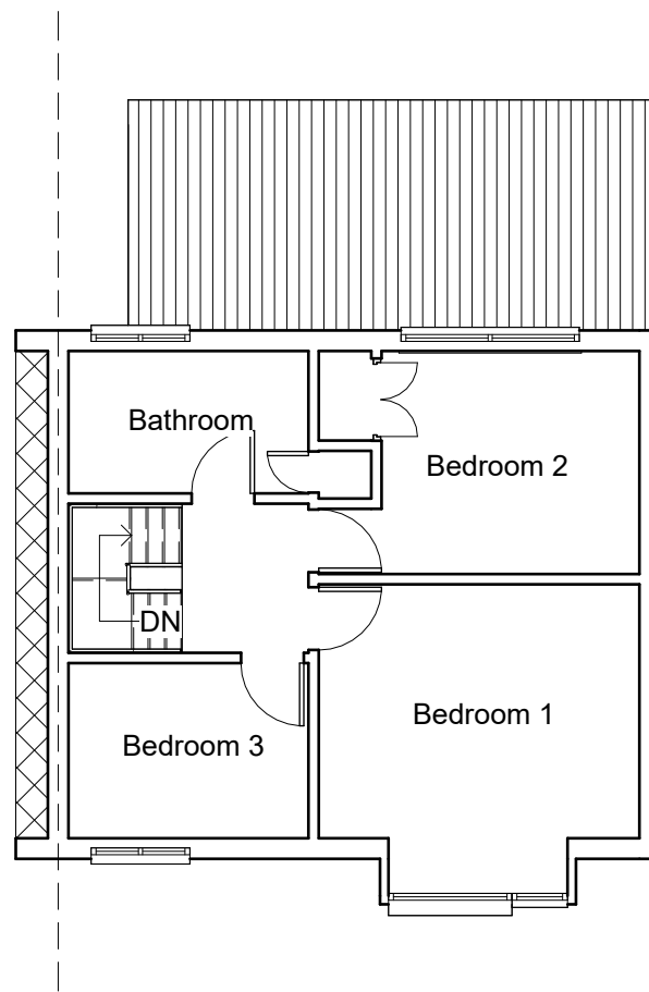
2 Existing First Floor 1 : 100
