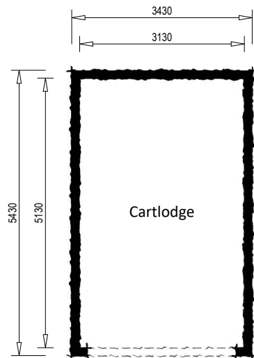
Floor Plan as Proposed
