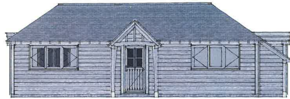
PROPOSED SOUTH-WEST ELEVATION
