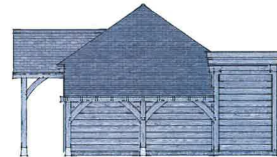
PROPOSED SOUTH-EAST ELEVATION
