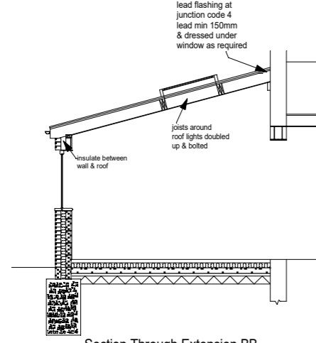
Section Through Extension BB
