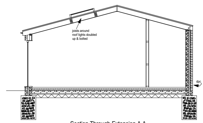
Section Through Extension A A
