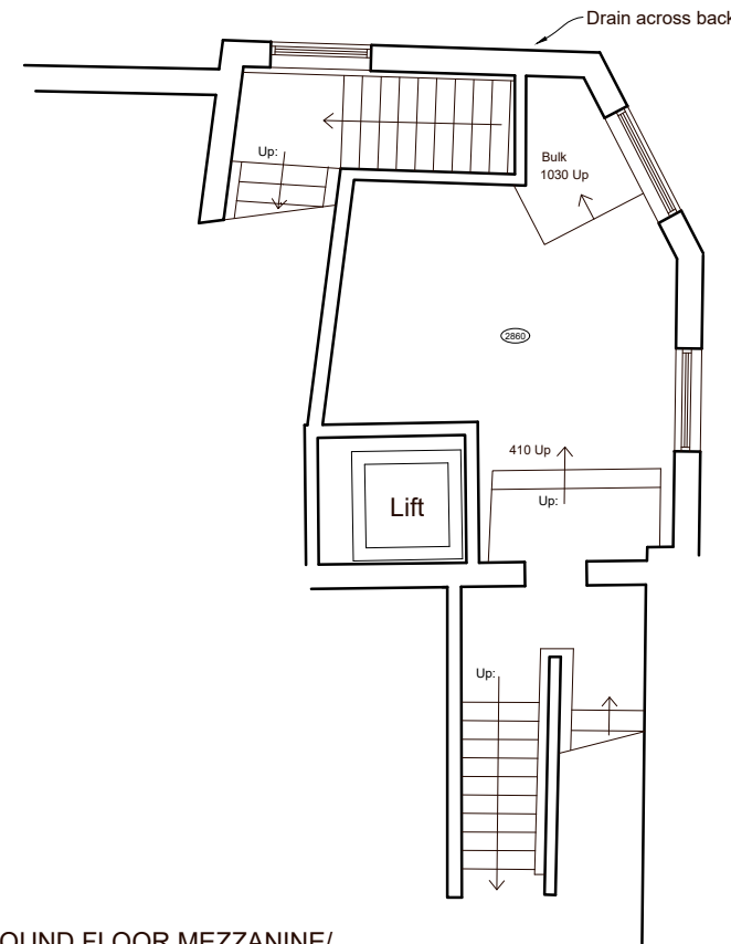
GROUND FLOOR MEZZANINE/ HALF LANDING PLAN
