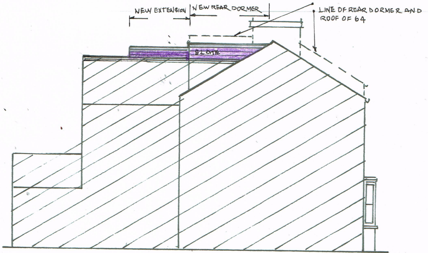
PROPOSED WEST ELEVATION "W"
