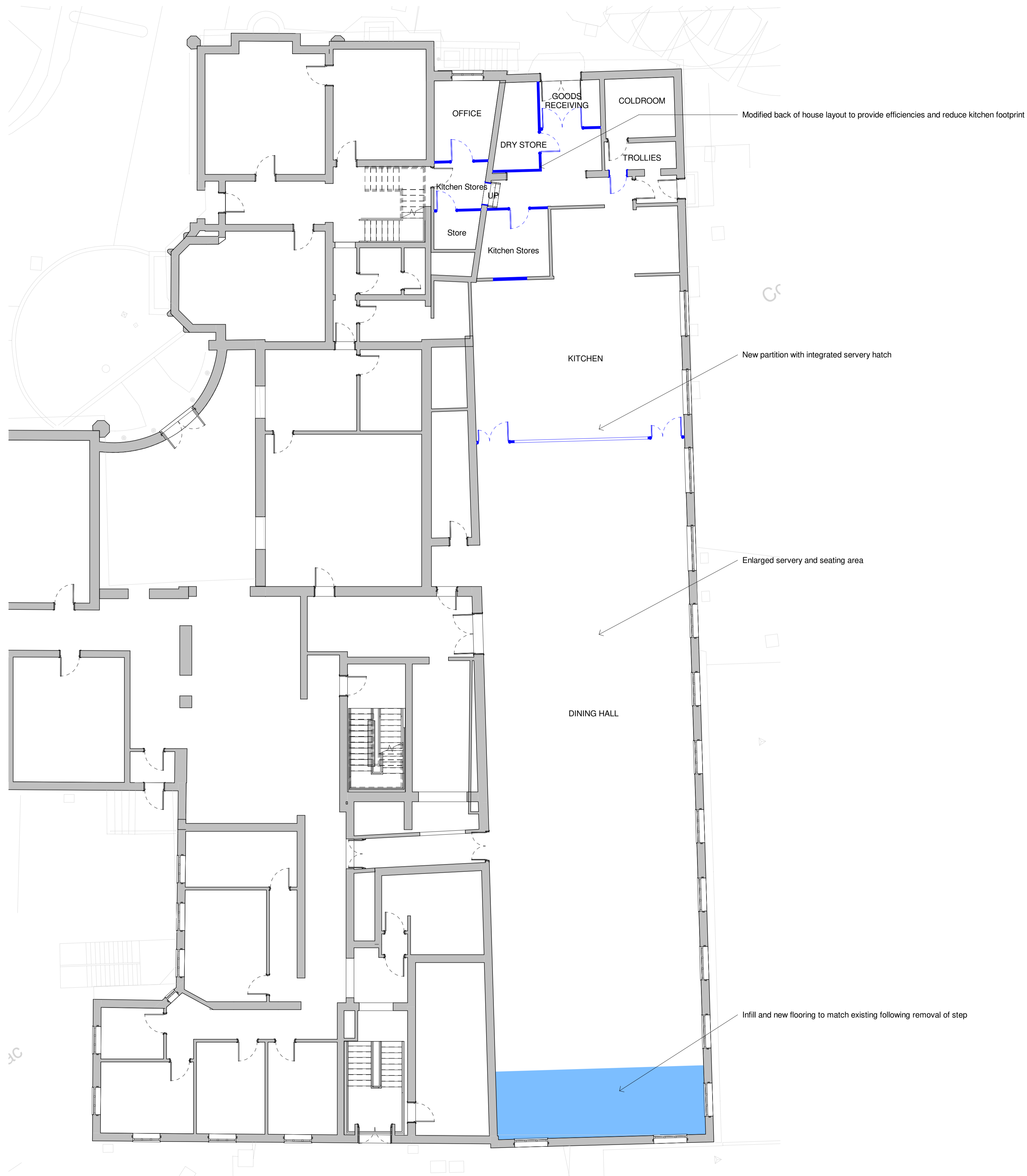
ZONE 07A PROPOSED PLAN 1 : 100
