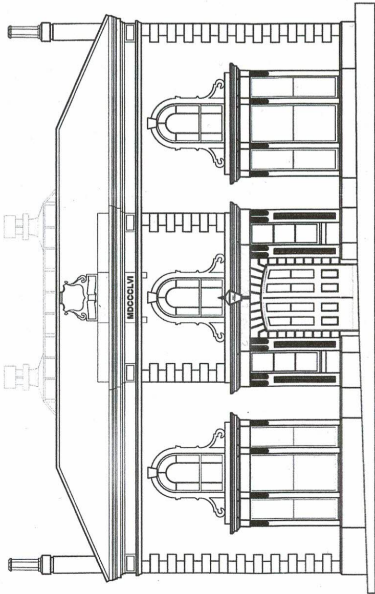
North Elevation - Existing 1:100
