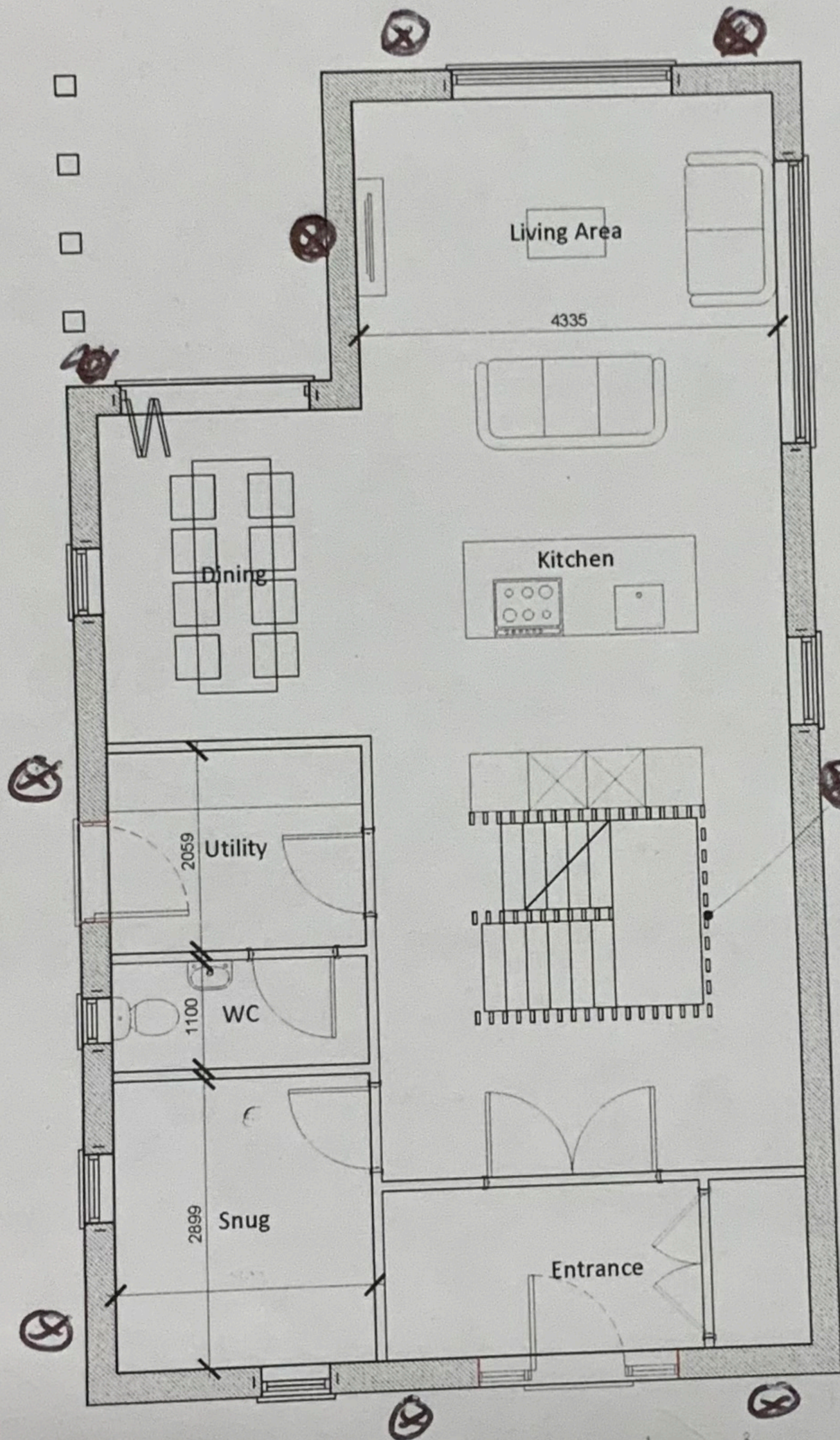
Ground Floor Scale 1:50
