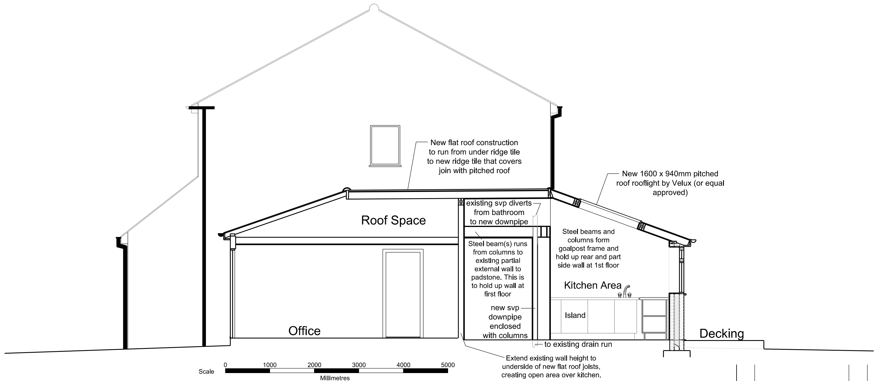
Proposed Side Sectional Elevation through Office and New Kitchen Area
