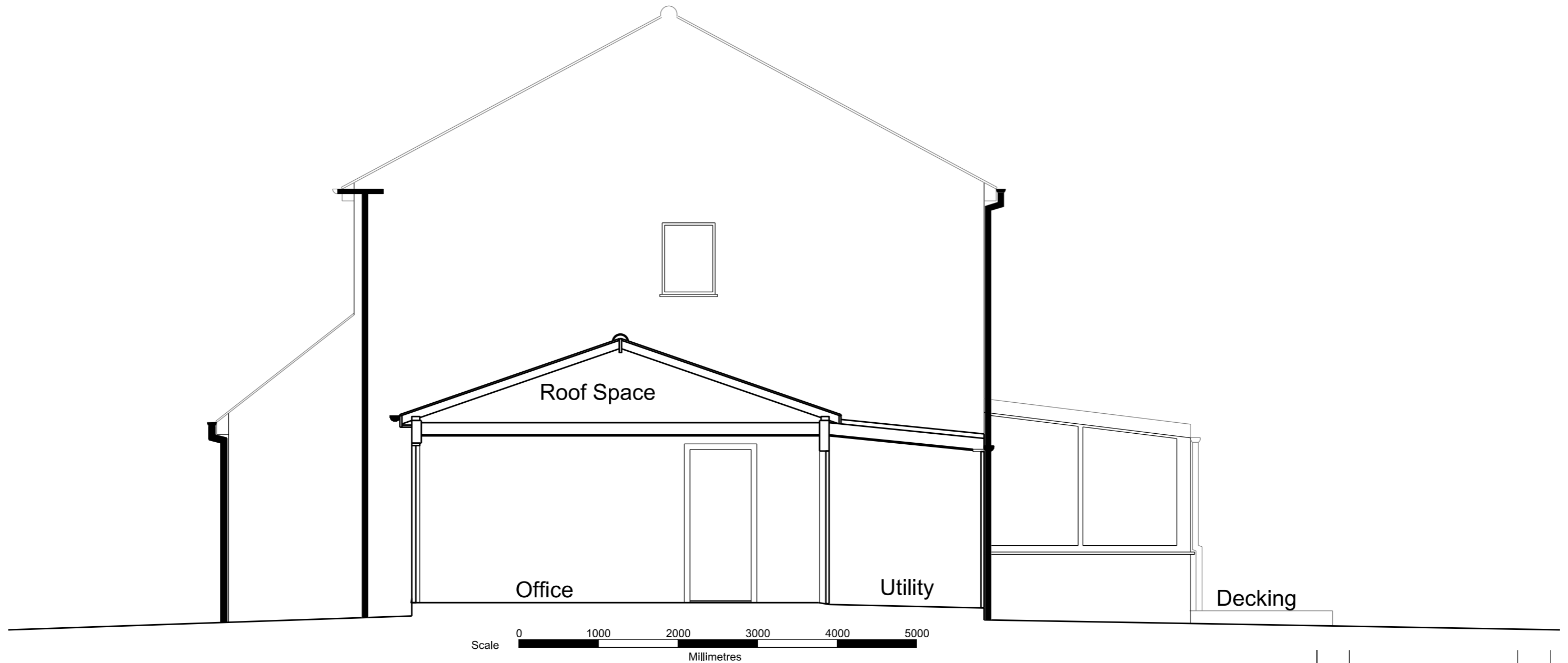
Existing Side Sectional Elevation through Office and Utility Room
