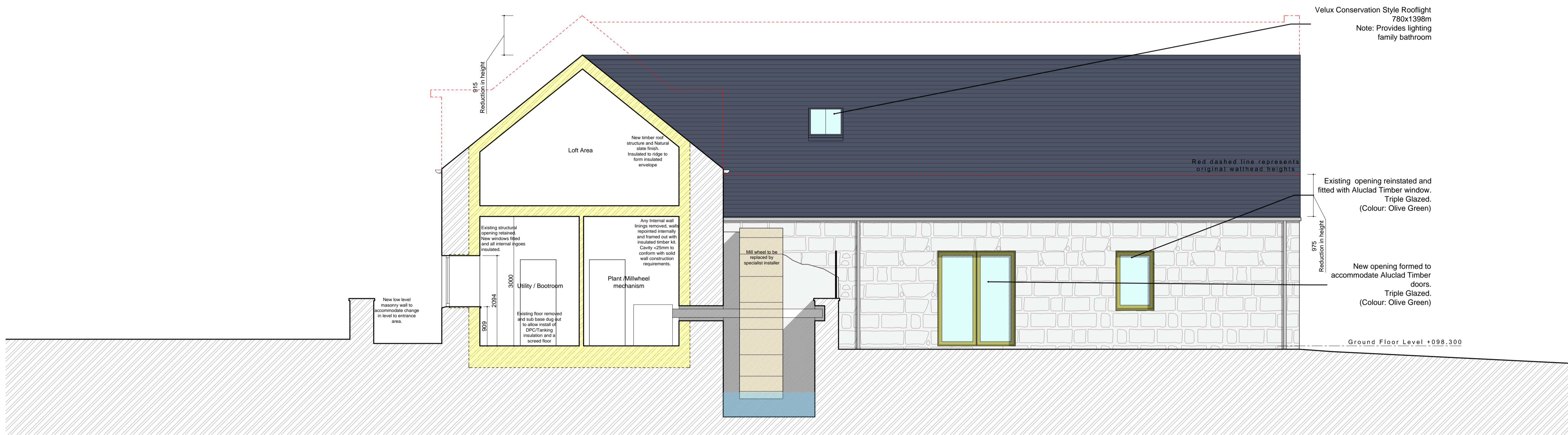
Proposed Section CC
