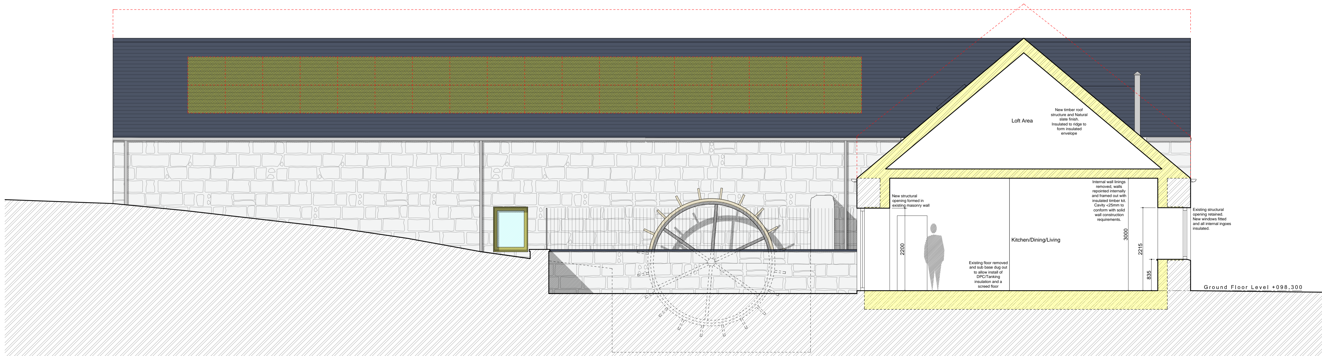
Proposed Section DD
