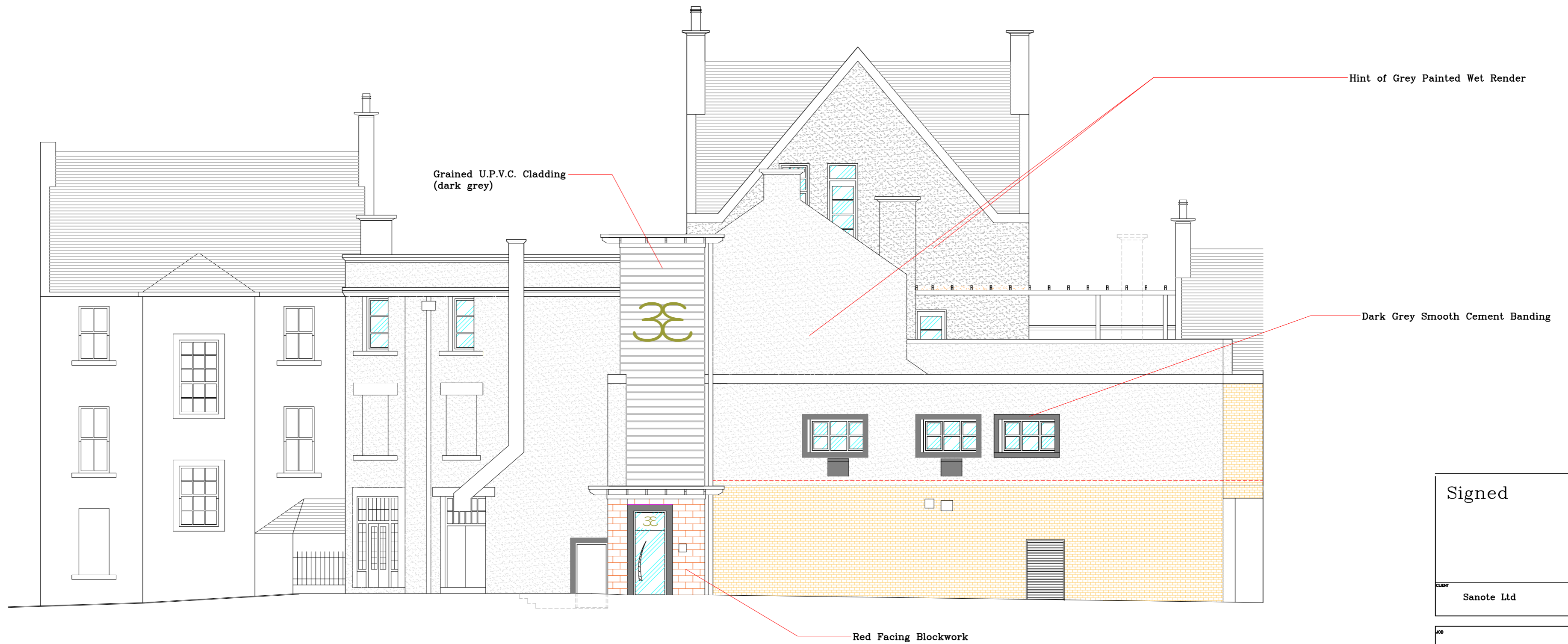
REAR ELEVATION – AS PROPOSED
