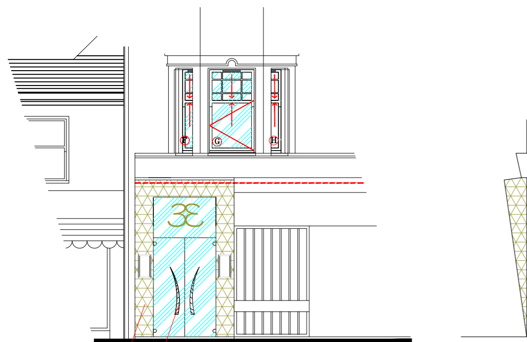
ENTRANCE DETAIL
