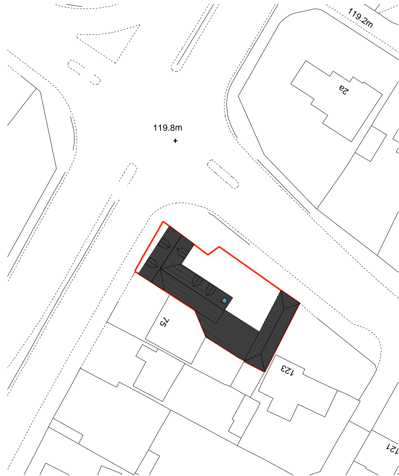
Block Plan 1:500
