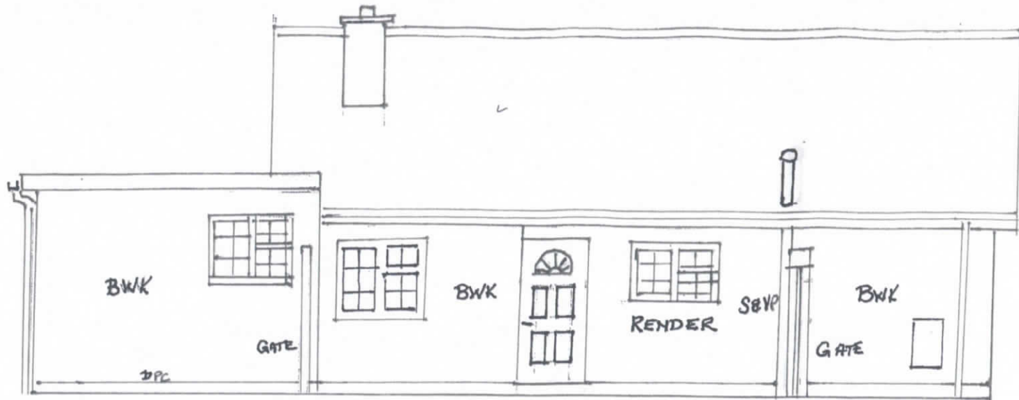
EXISTING NORTH ELEVATION (REMAINS) Scale: 1.50
