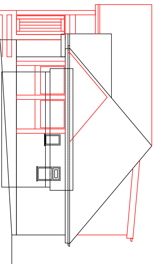
South East Elevation Comparison
