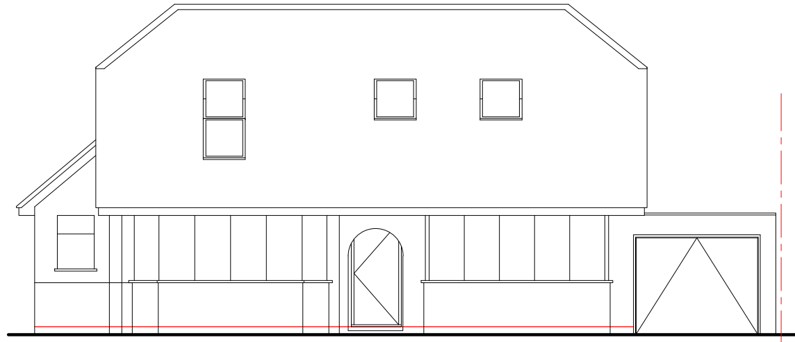
EXISTING FRONT (SW) ELEVATION
