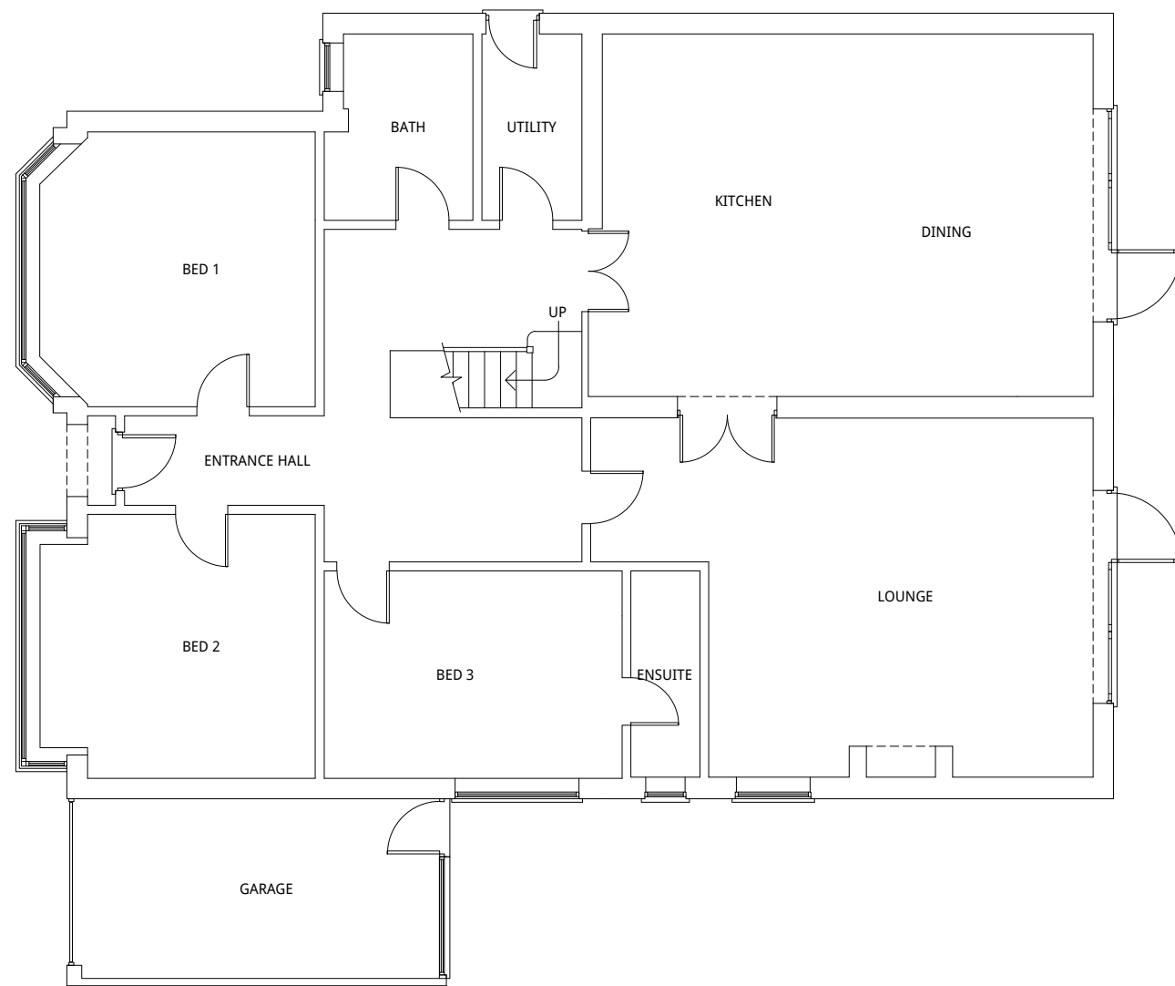
EXISTING GROUND FLOOR PLAN (NO CHANGES PROPOSED)
