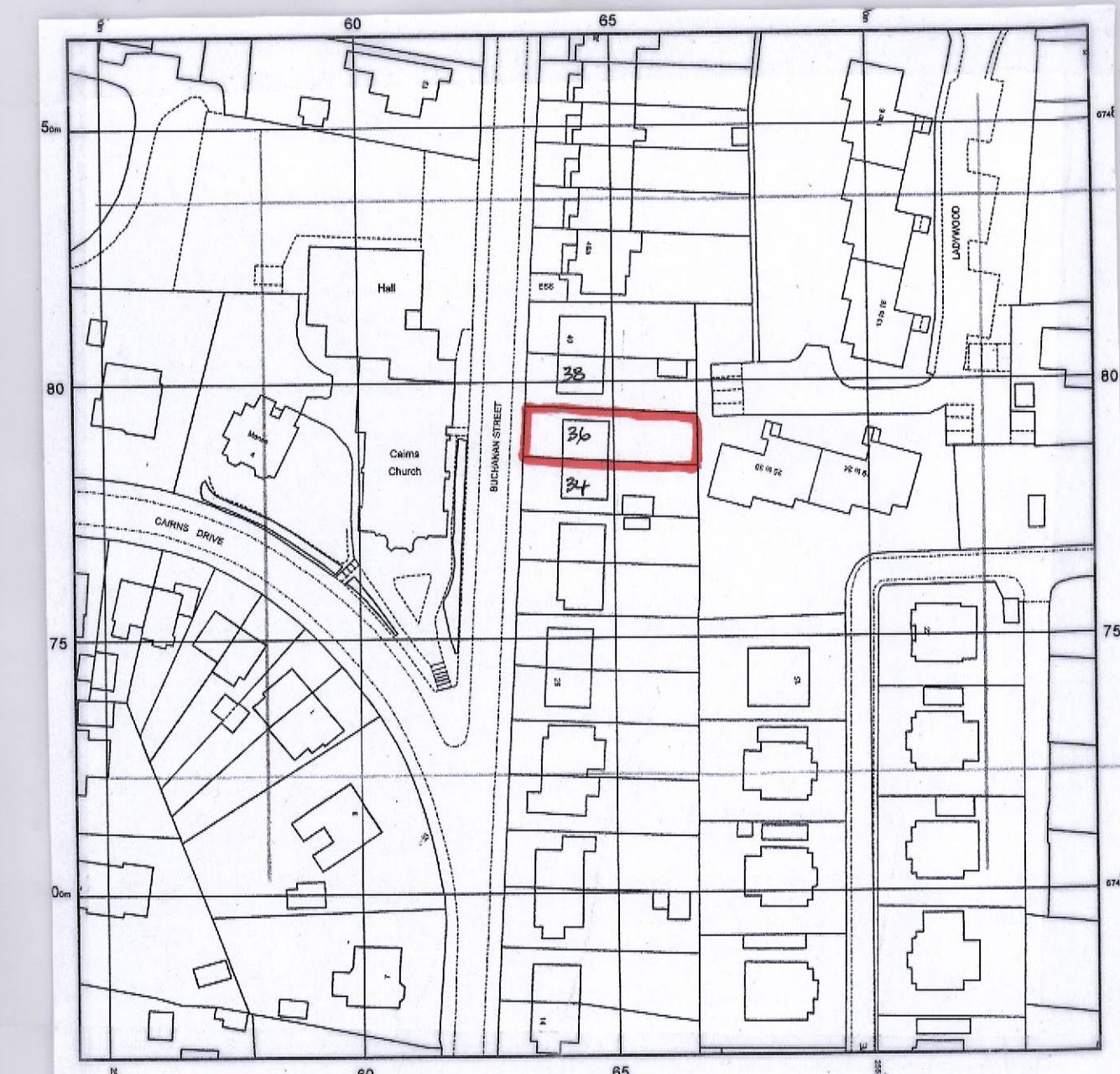
Location Plan 1:1250.
