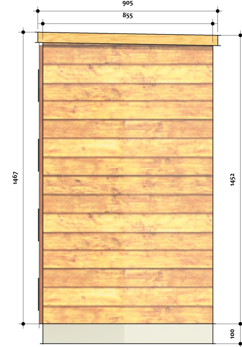
5 RIGHTSIDE ELEVATION - BIN SCALE 1 : 10 SHEET REF:
