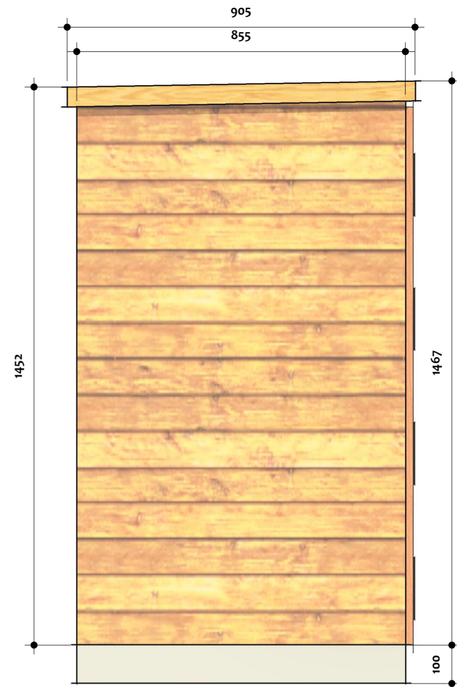
5 RIGHTSIDE ELEVATION - BIN SCALE 1 : 10 SHEET REF:
