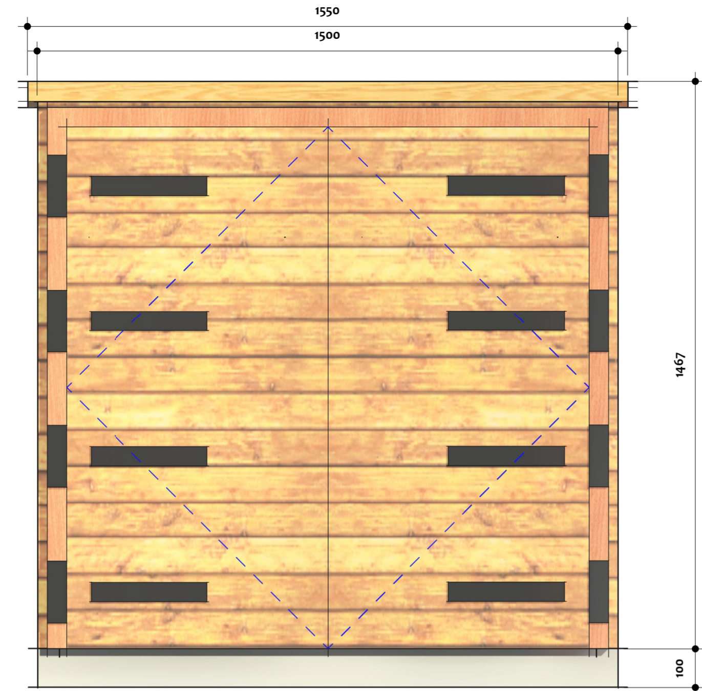
3 FRONT ELEVATION - BIN SCALE 1 : 10 SHEET REF:
