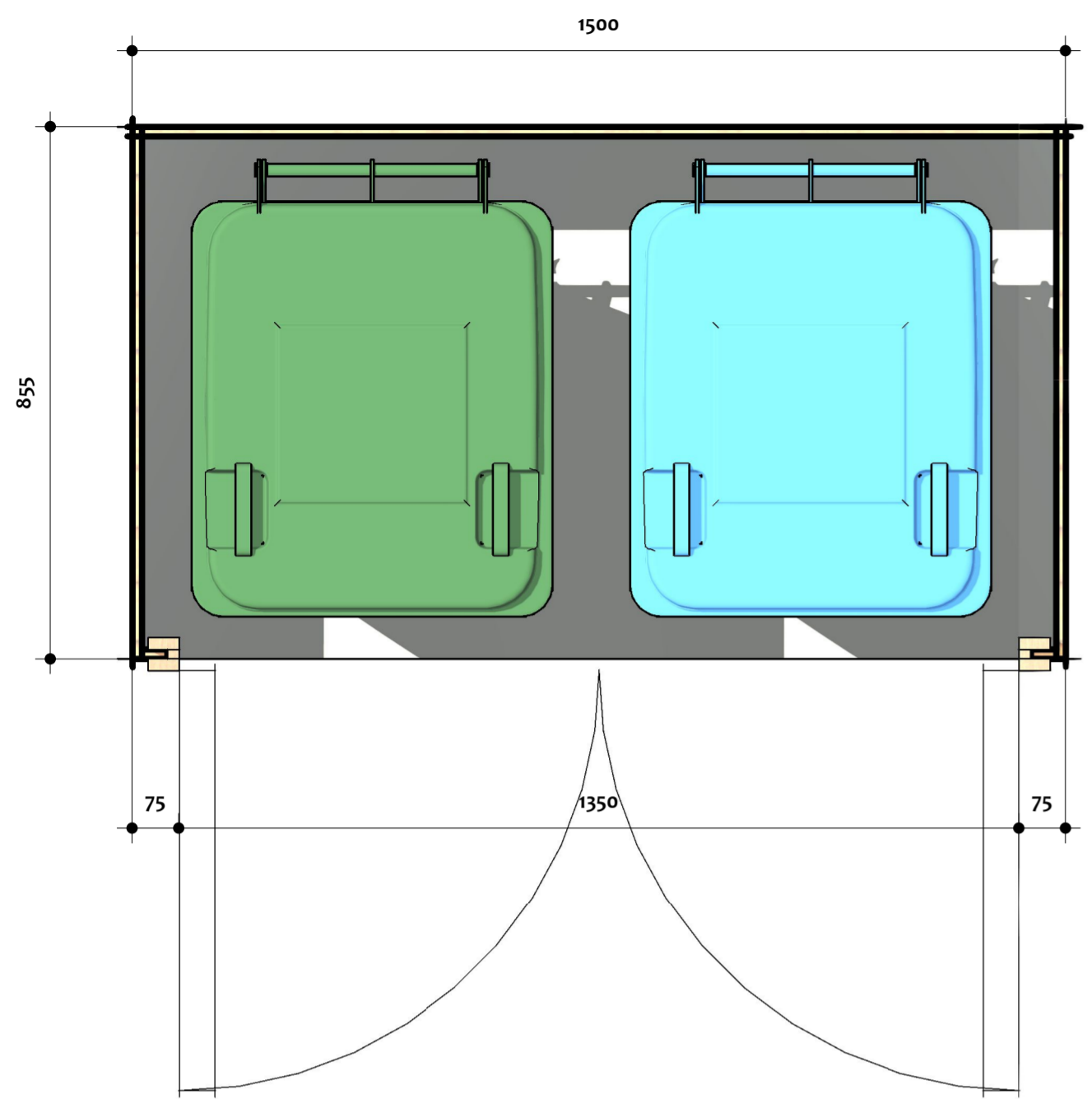
1 BIN SHED SCALE 1 : 10 SHEET REF: A107
