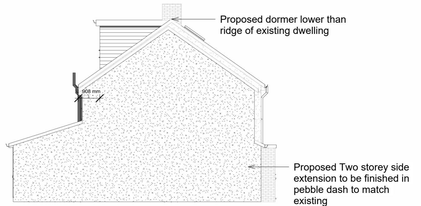
PROPOSED SIDE B ELEVATION
