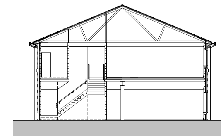
Short Section
