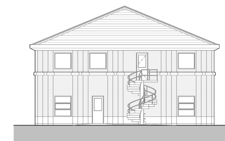
South Elevation A - North Elevation G
