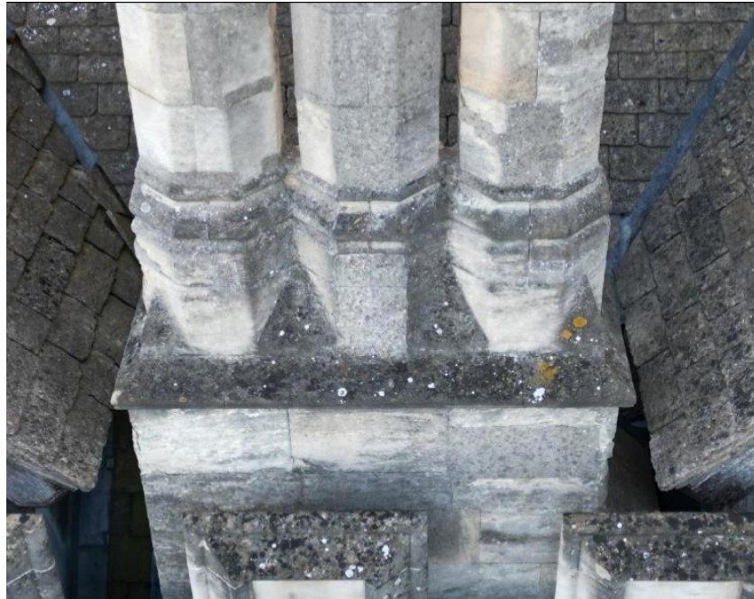
Fig. 5 Base of Chimney stacks – High Street elevation
