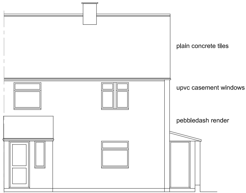
FRONT ELEVATION
