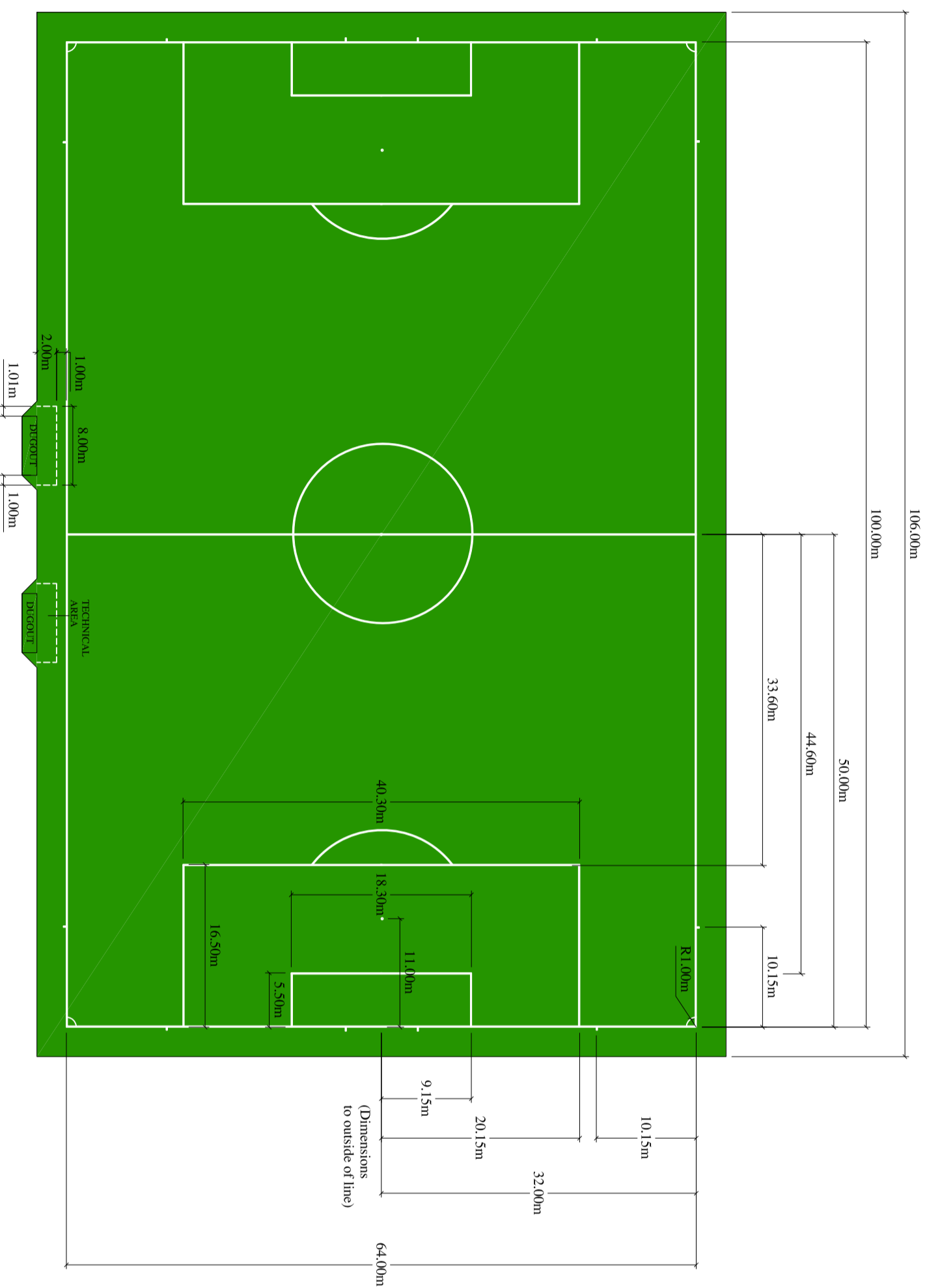
LINE MARKING - 1:500
