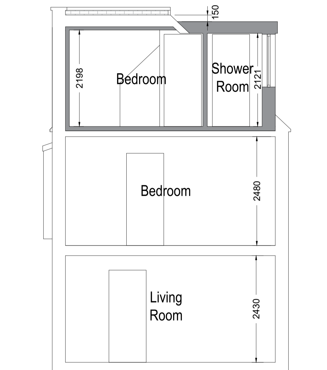
Section A-A Scale 1:50
