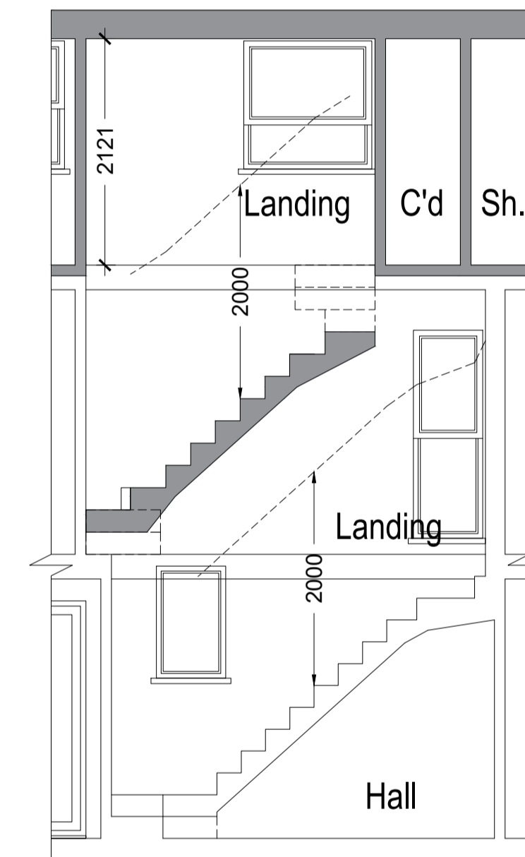
Section B-B Scale 1:50
