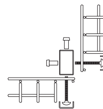
Plan of external corner
