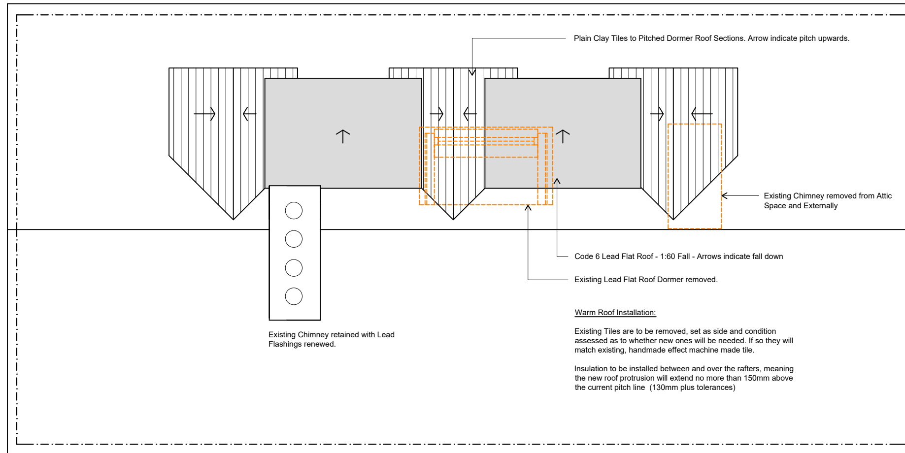
Proposed Main Roof Plan 1:50
