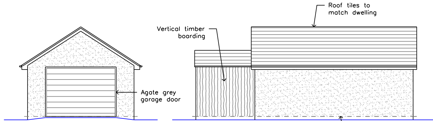
SIDE ELEVATION
