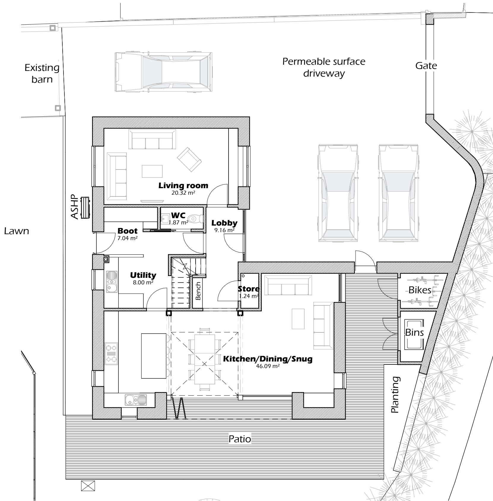
1 Ground Floor 1 : 100
