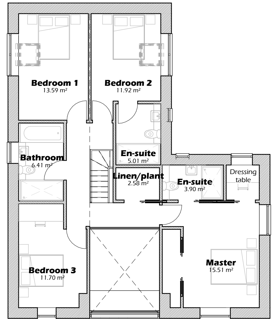
2 First Floor 1 : 100
