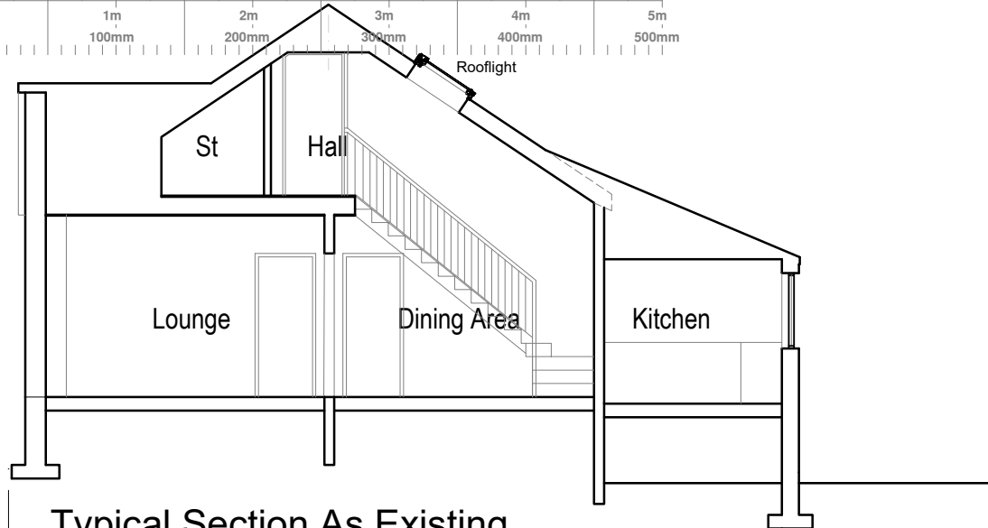
Typical Section As Existing
