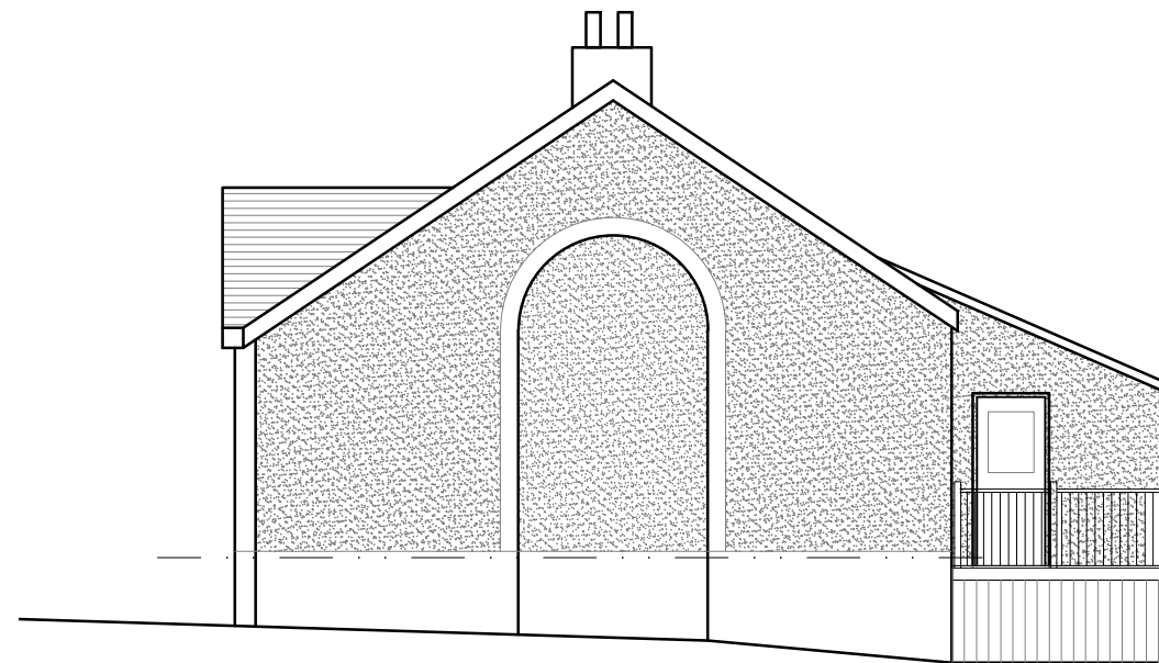
Gable Elevation As Existing To Neighbours
