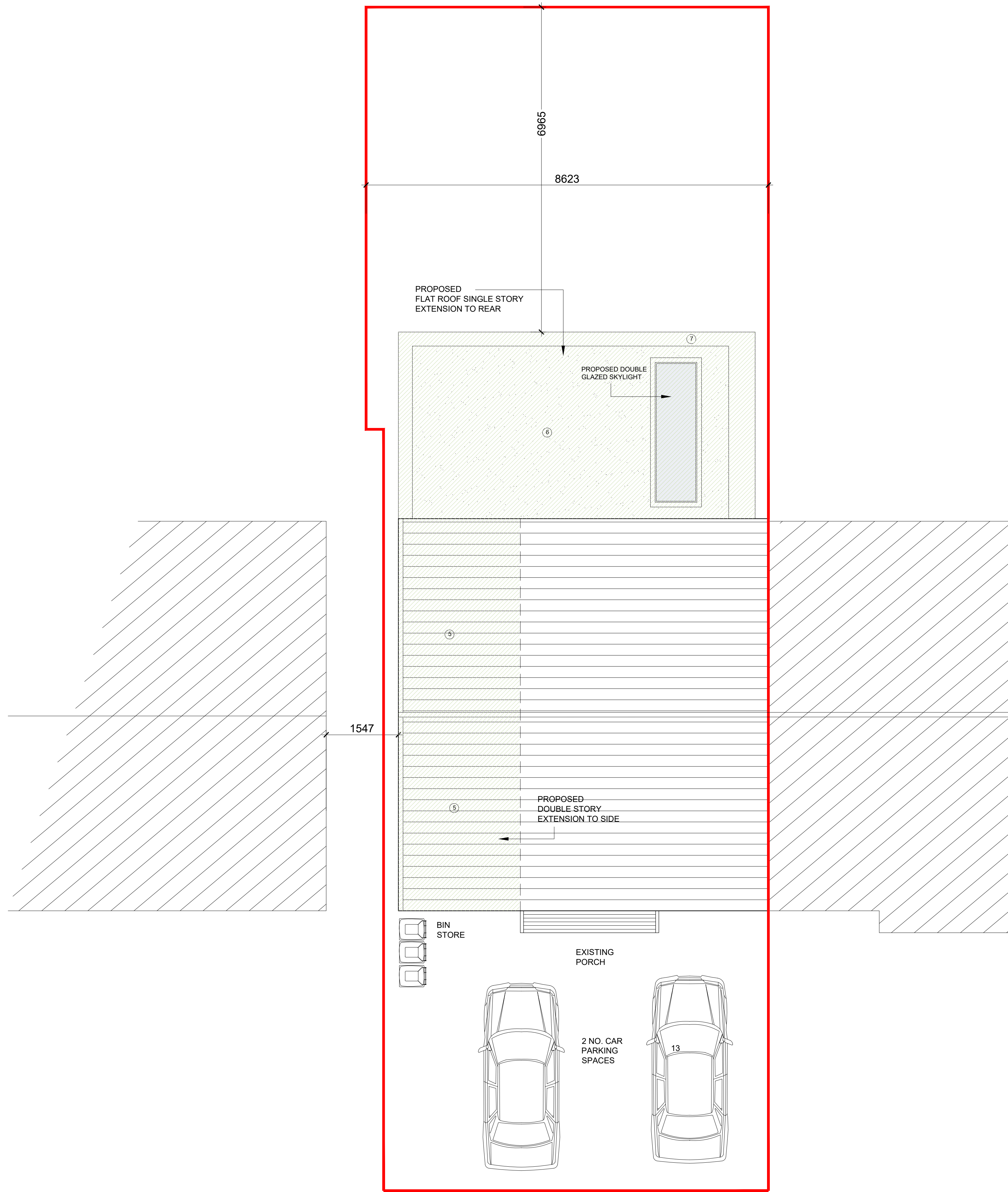
① PROPOSED SITE PLAN
