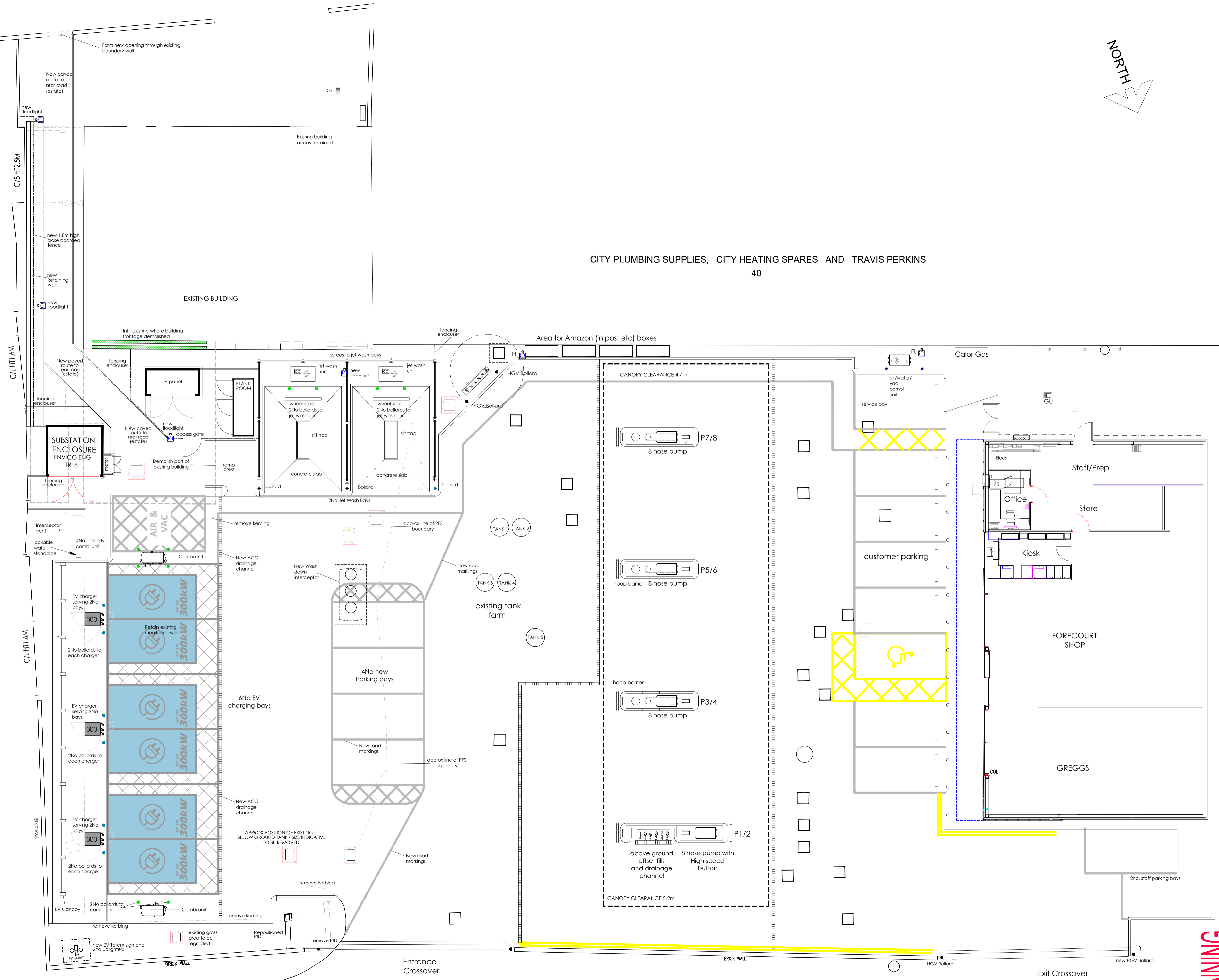
Proposed Site Layout Plan Scale 1:100
