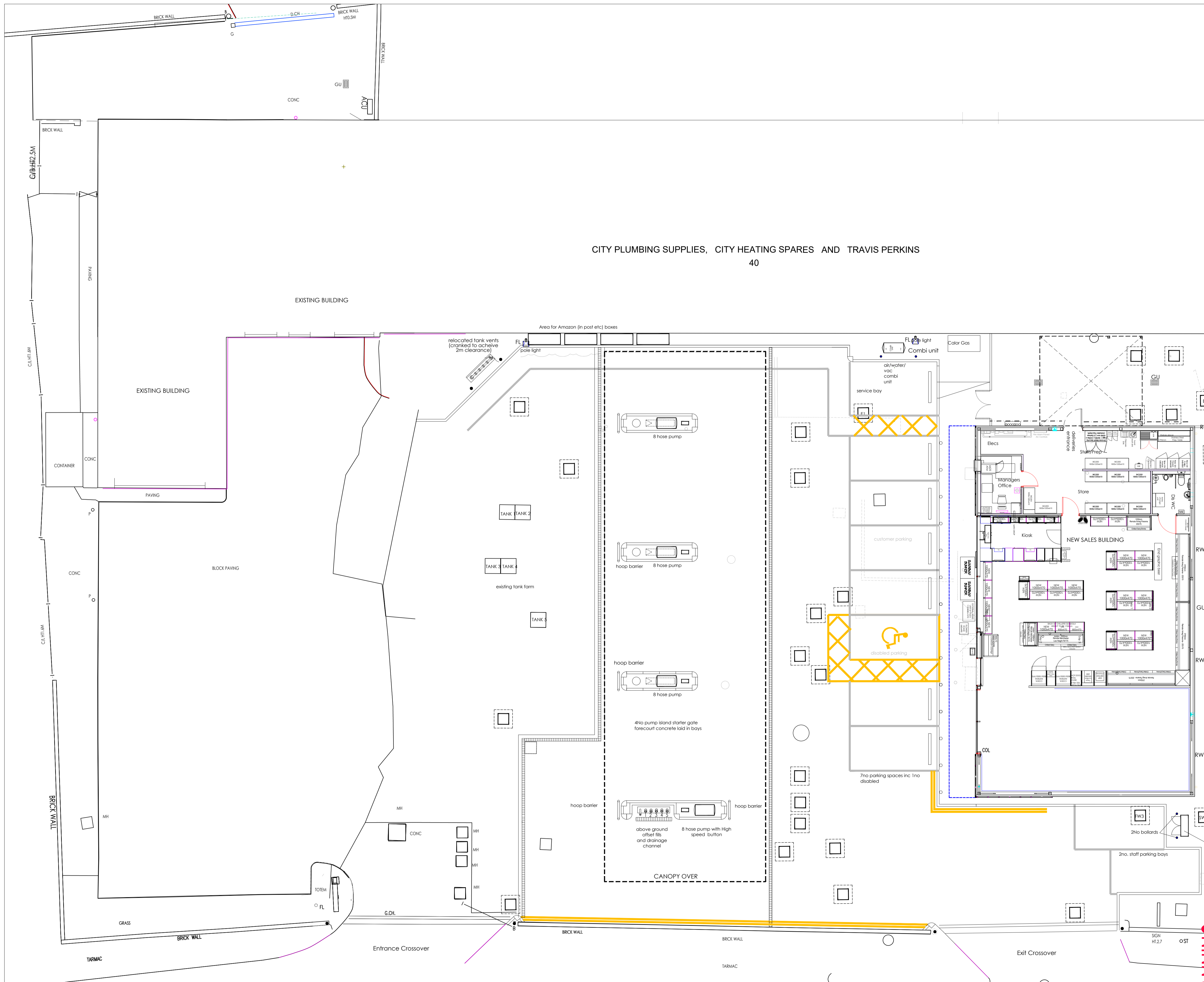
Existing Site Layout Plan Scale 1:100
