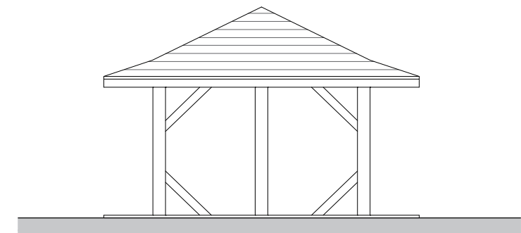
Side (East & West) Elevations
