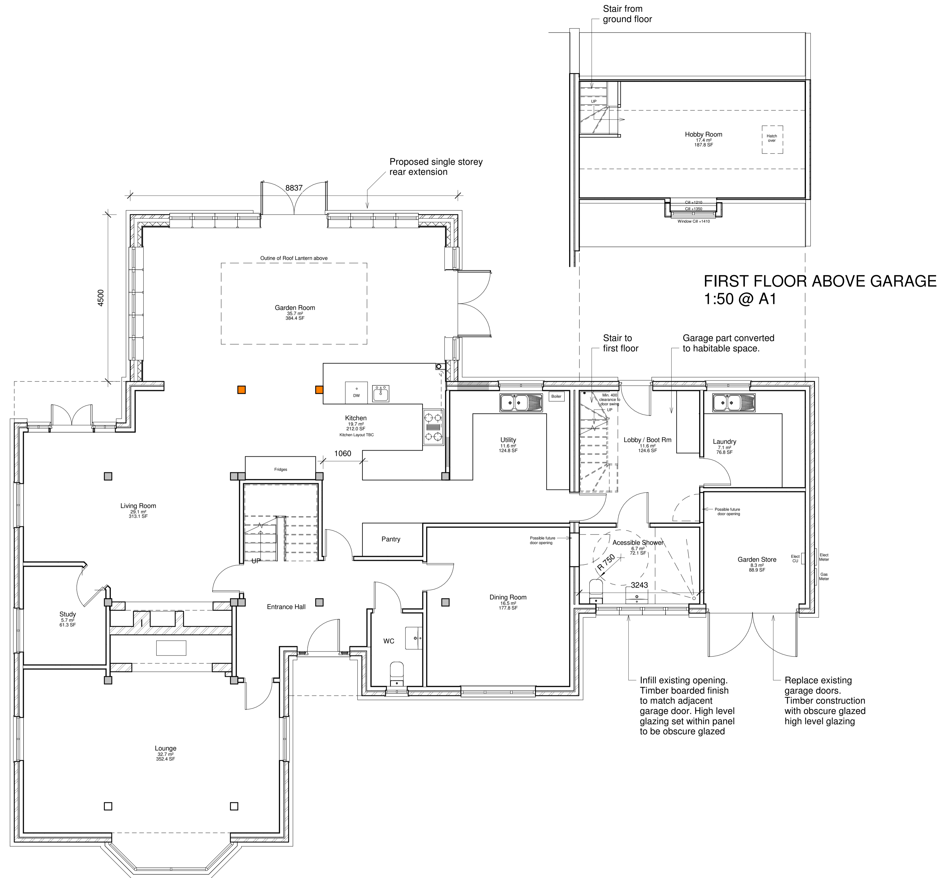
GROUND FLOOR PLAN 1:50 @ A1
