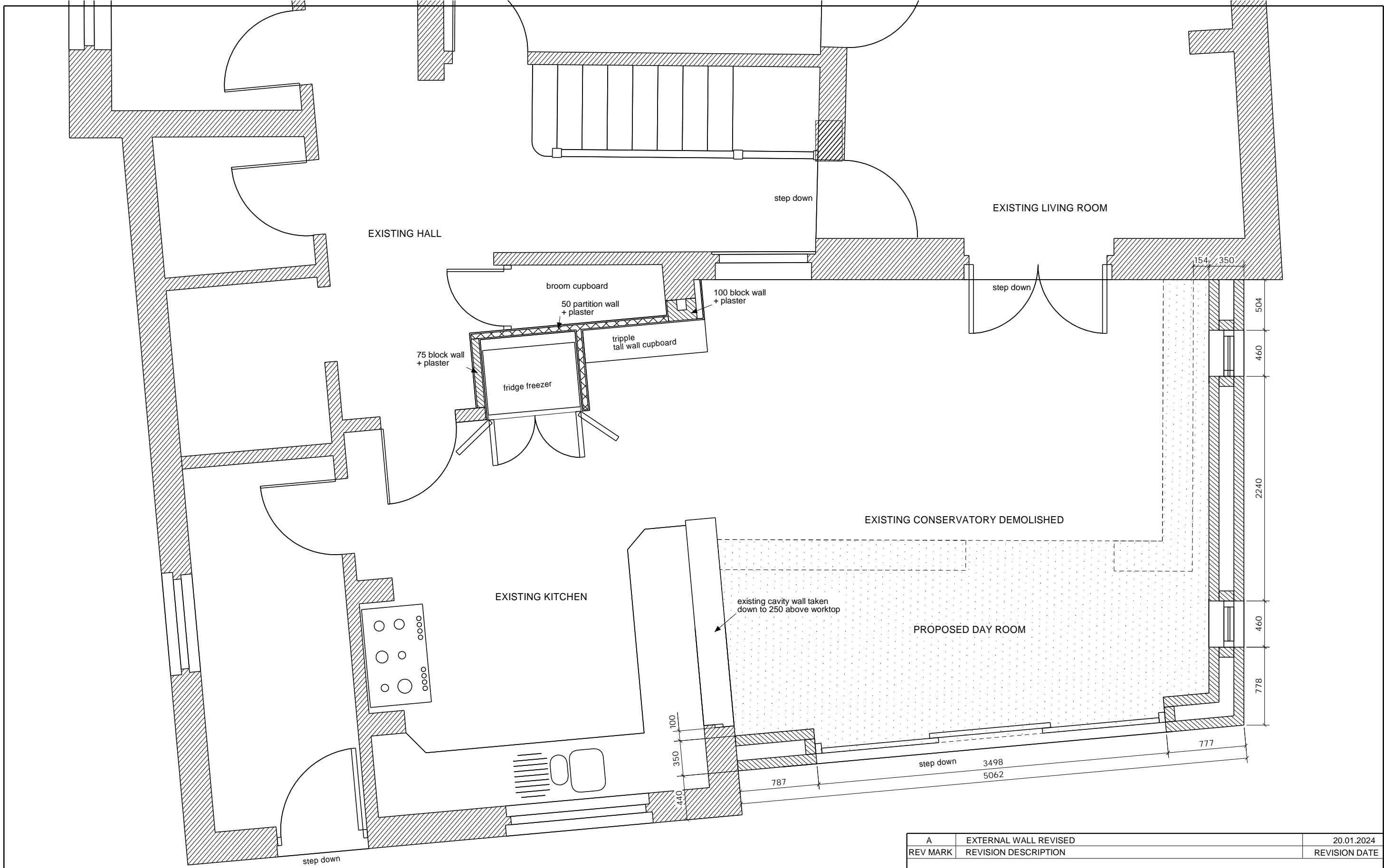
PROPOSED GND FLOOR PLAN
