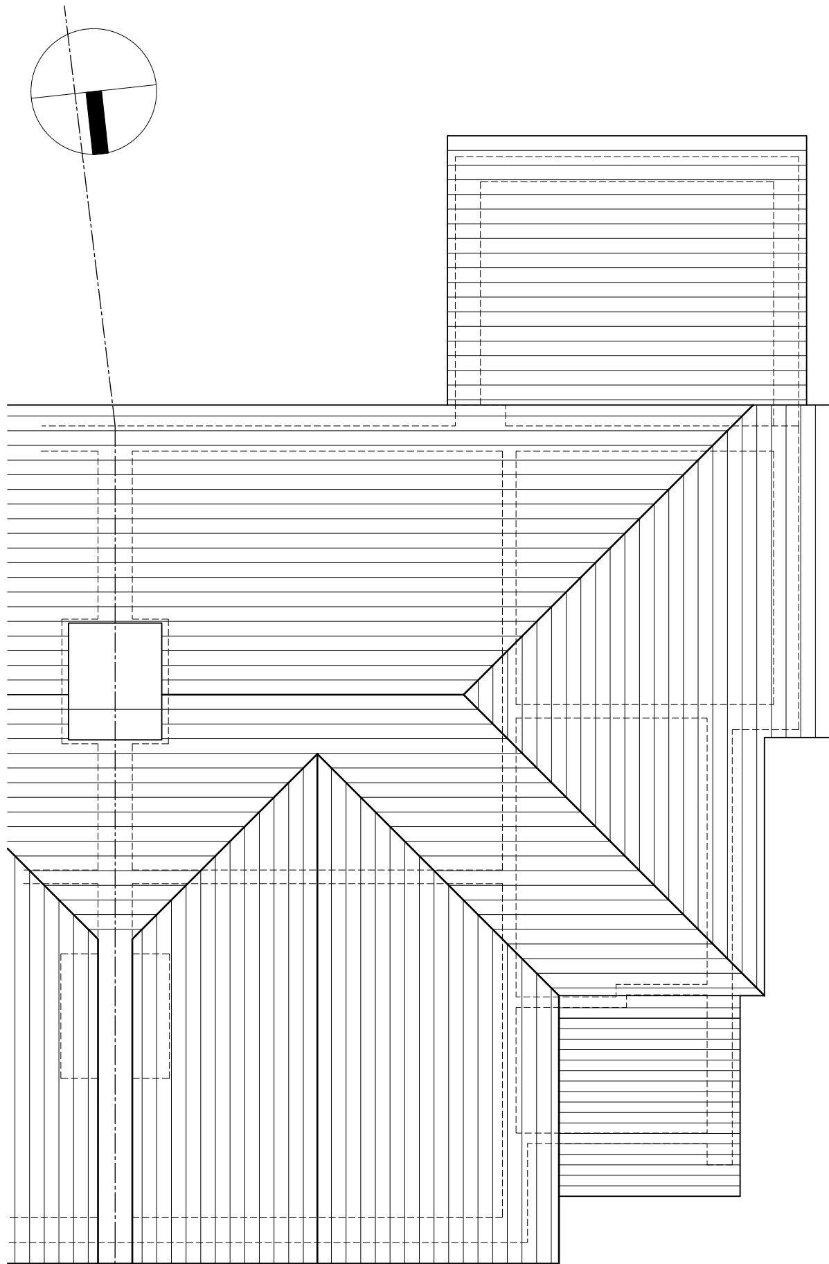
ROOF PLAN 1:50
