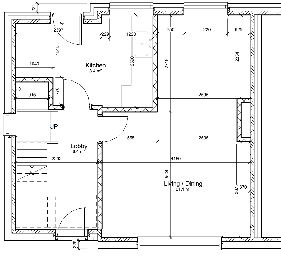
00 - Ground Floor GA 1 : 50
